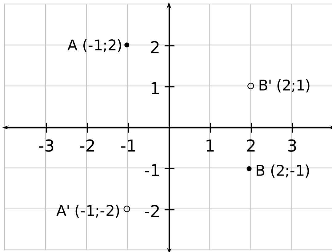
Figure 13.43: Points A and B are reflected on the x -axis. The original points are shown with \bullet and the reflected points are shown with \circ .
