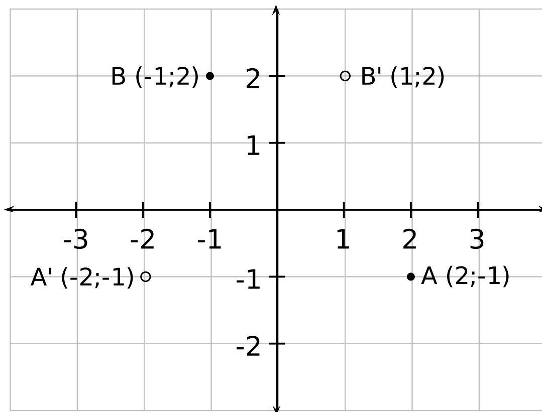
Figure 13.44: Points A and B are reflected on the y -axis. The original points are shown with • and the reflected points are shown with ○.
